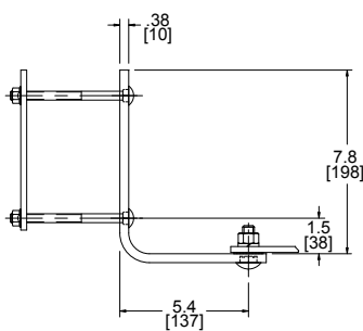
Extended bracket
